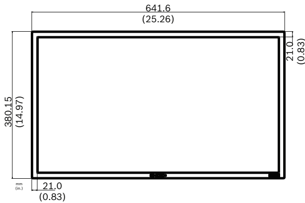
UML-273-90: Front View
